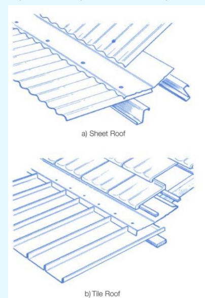
Figure 3: Change of pitch flashing
