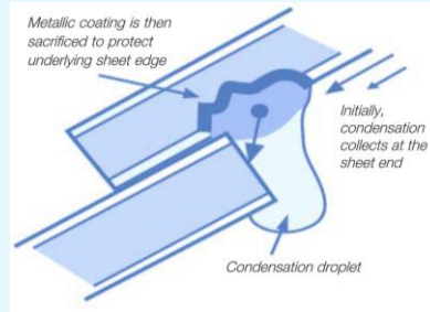
Figure 1: Cross section of sheet lap
