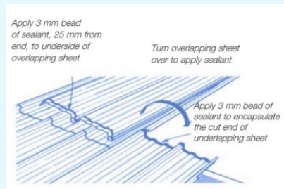
Figure 2: Sealant position recommendation
