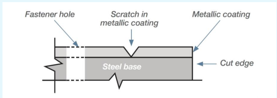
Figure 1: Schematic of a cut edge (not to scale)
